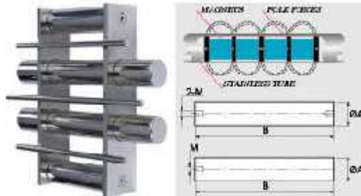
Magnetic filter
